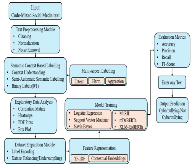
Figure 5-Model Architecture
